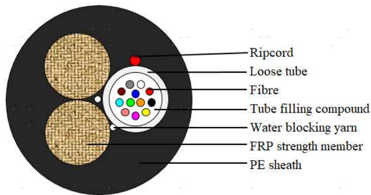
GYFY(3U)-12B1.3 Schematic for reference only
